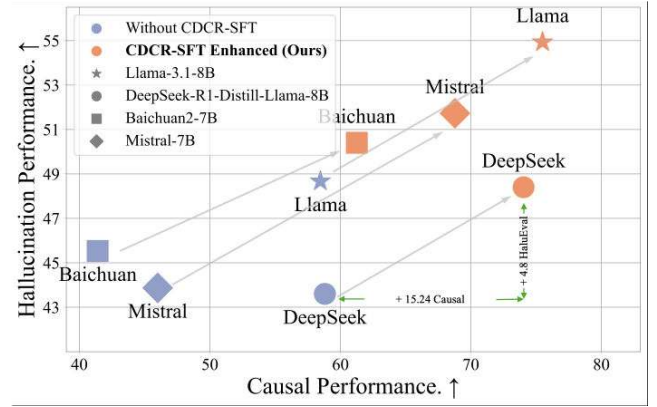
Figure 1: Average overall performance of our CDCR-SFT applied to four LLMs on the causal reasoning benchmarks (CLADDER and WIQA) and the hallucination benchmark (HaluEval). Orange symbols mark LLMs enhanced by CDCR-SFT, showing clear gains in causal reasoning and reduced hallucinations.
