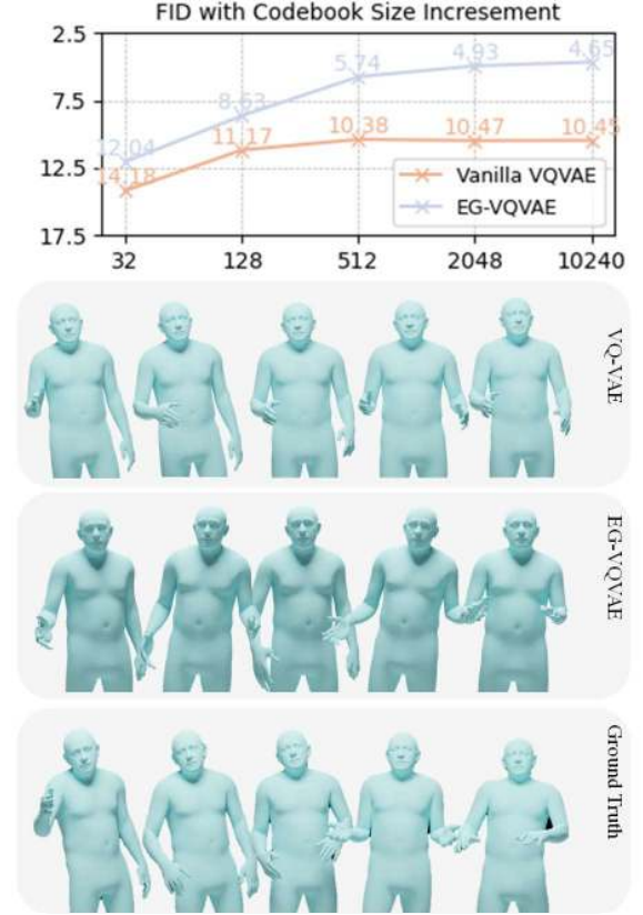
Figure 7: Impact of Codebook Size. Contrary to the vanilla gesture VQ-VAE, EGGesture continues to benefit from an increase in codebook size. Results demonstrate a increase in codebook size will have an improvement on FID; subjective visualization further shows our method can capture more refined motion representations. e.g. raising the same hand as the groundtruth. FID results are evaluated on BEAT with fixed latent vector length 256.
