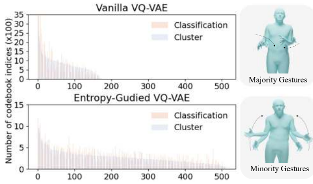
Figure 1: Distribution of Codebook Indices. Top: Vanilla gesture VQ-VAE illustrates an imbalanced distribution with 28% utilization for a codebook of size 512, resulting in an audio-predicted gesture bias towards majority classes. Bottom: Through entropy regularization, our Entropy-Guided VQ-VAE method ensures maximized utilization and a balanced distribution, yielding a classification result that aligns closely with both majority and minority classes.
