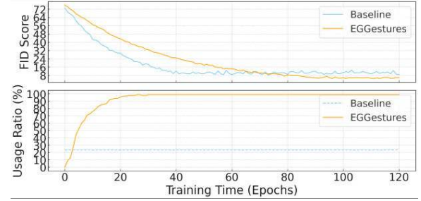
Figure 6: Usage Ratio of Codebook. we show both the codebook usage ratio and FID Comparison for baseline and our method, note that baseline use a fixed codebook raito for stage-two.
