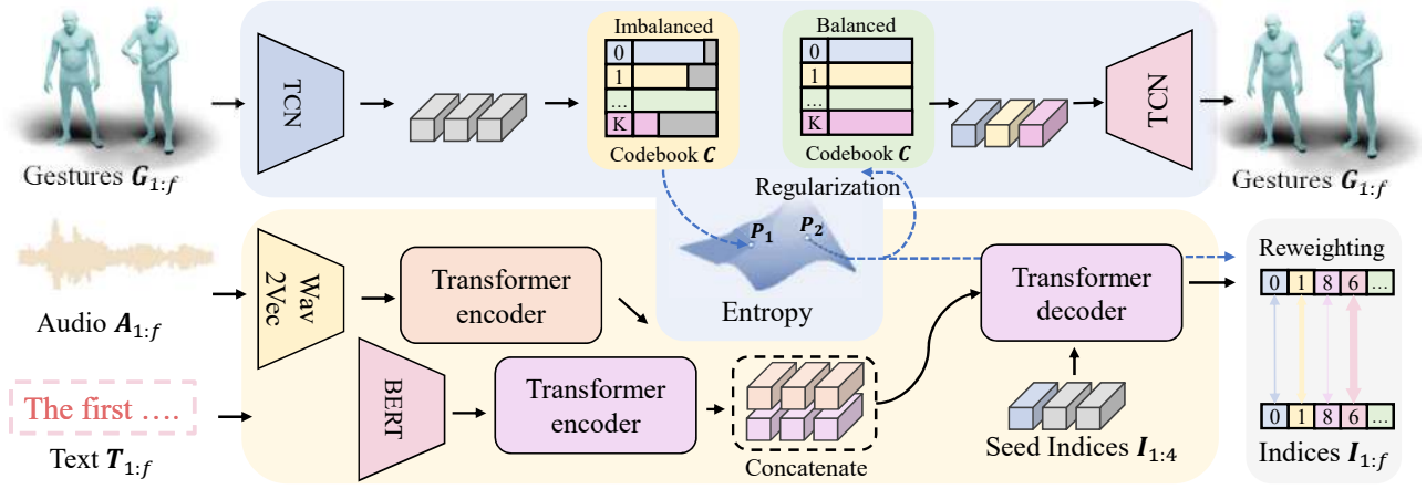
Figure 3: Overview. EGGesture performs jointly differentiable optimization of gesture codebook learning and audio-to-codebook classification. Top: Gesture motions are translated into latent vectors, matched to the closest codebook vector, with reconstruction through the decoder. Bottom: Pre-trained audio and text features, derived from wav2vec and BERT, proceed through a transformer encoder and merge via channel-level concatenation. Subsequent classification to codebook indices is managed by a transformer decoder. Middle: Codebook entropy, determined by the cosine similarity between continuous and quantized latents alongside Gumbel Softmax, is maximized during training. The entropy guides two optimizations: i) Balancing codebook distribution for refinement utilization and ii) Reweighting codebook indices to refine classification loss for improved audio-to-motion classifications.
