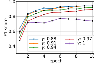
Figure 10: Effect of discounted rate \gamma . With \gamma = 0.88 BLECS performs optimally.
