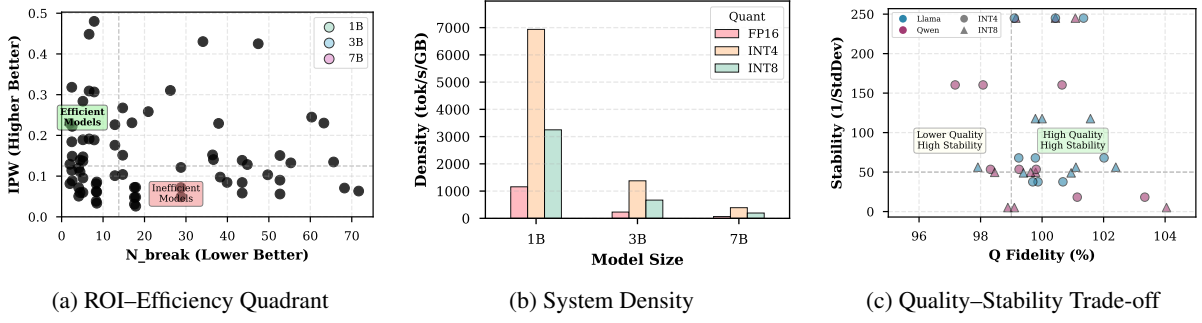
Figure 3: Multidimensional efficiency under legacy deployment—compact ( < 2B ) models form the ROI-IPW efficiency frontier, INT4 enables a strong throughput-per-GB hardware multiplier, and quantization fidelity remains stable with controlled variance.
